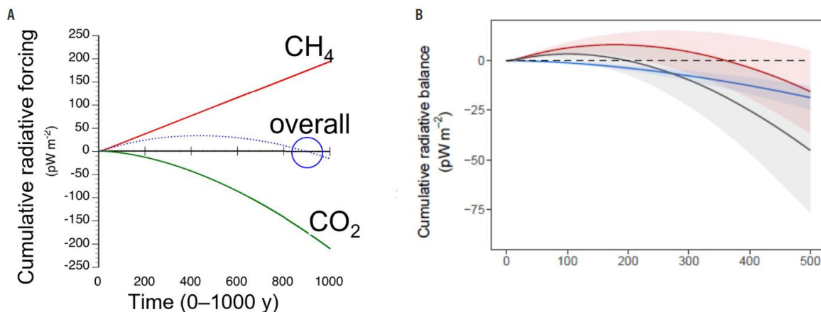
Figure 3. Cumulative radiative balance and cross-over times from net warming to net cooling effects. Radiative forcing is the impact that different factors, such as GHG, have on the balance of incoming and outgoing energy in the Earth's atmosphere. The cumulative radiative forcing is described as the difference between the warming effect of methane emissions and the cooling effect of carbon dioxide sequestration. A) The cross-over point for a freshwater tidal marsh in Virginia is depicted by the blue circle and is the time when the cumulative radiative forcing transitions to negative. B) Cross-over times are influenced by salinity. The tidal wetland (blue) is negative from inception, where the nontidal restoration sites (red and black) reach a net zero cumulative radiative force at 200 to 400 years after inception. Figure taken from Windham-Myers et al. (2023).
