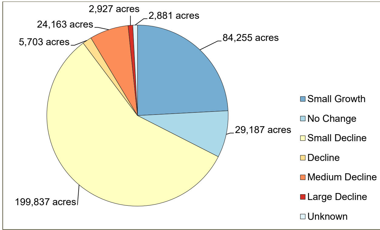
Figure 2.1 Delta Crop Yield Impacts Under Climate Change, Based on predictive modeling for temperature change in California.
